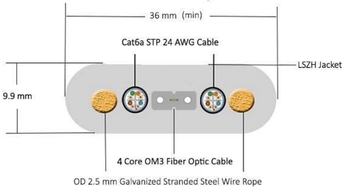
Industrial Flexible Elevator Cable 2 x Cat6a STP 24 AWG Cable + 4 Core OM3 Fiber Optic Cable
