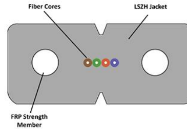
4 Core OM3 Tight Buffered Multimode Fiber Optic Cable
