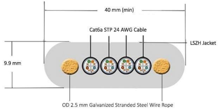
Industrial Flexible Elevator Cable 4 x Cat6a STP 24 AWG Cable
