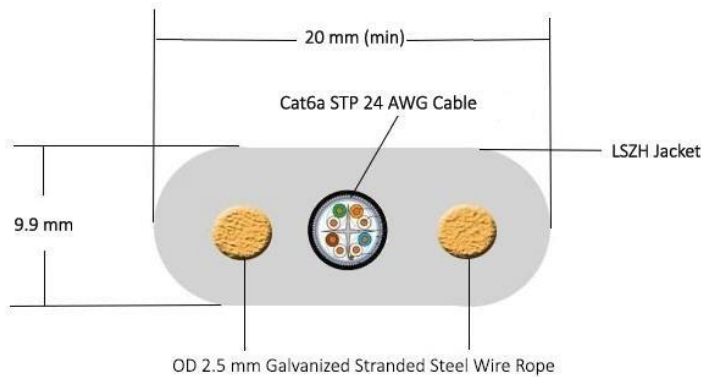
Industrial Flexible Elevator Cable 1 x Cat6a STP 24 AWG Cable
